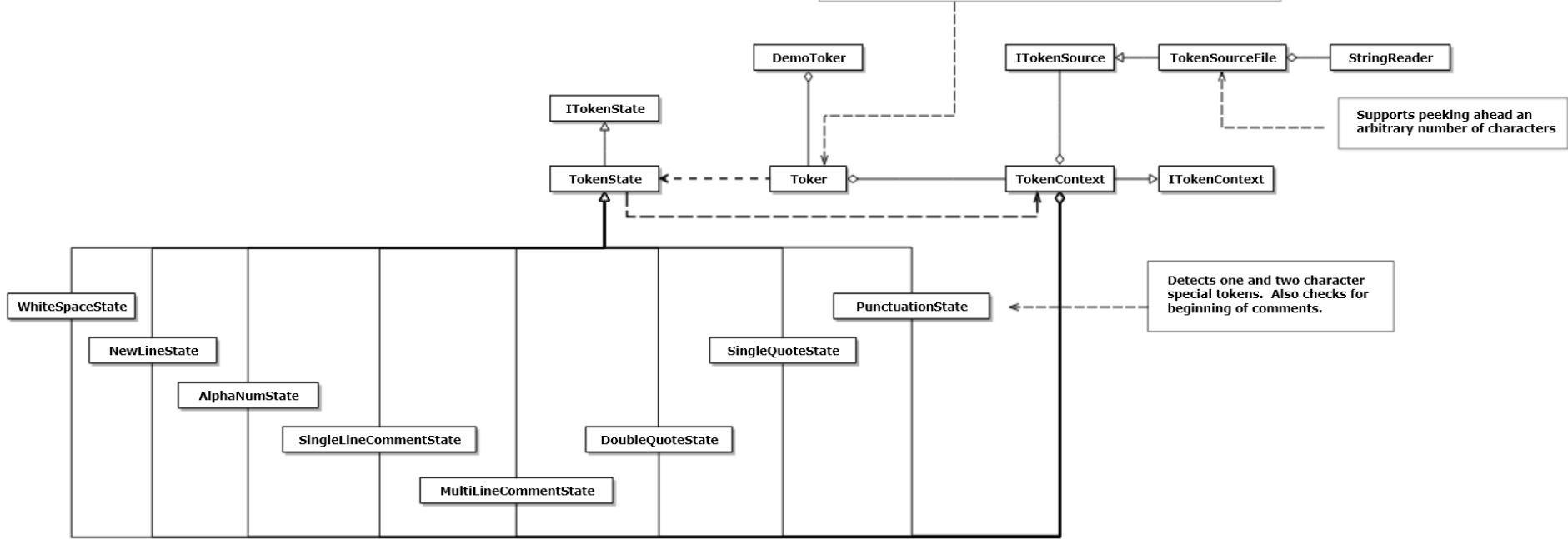
StatePattern_Toker Class Diagram
