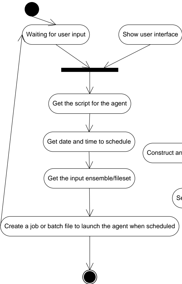
Activity Diagram - Providing Input for Agent
