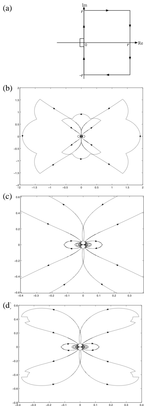
Fig. 4. (a) The Nyquist path \mathcal{D}^\theta ; (b) Nyquist plot for \theta = 0 ; (c) Blown-up version of plot in (b); (d) Nyquist plot for \theta = 0.5 .
