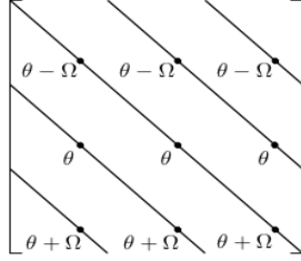
Fig. 3. Interpretation of \mathcal{G}_\theta as “samples” of \hat{G} .
