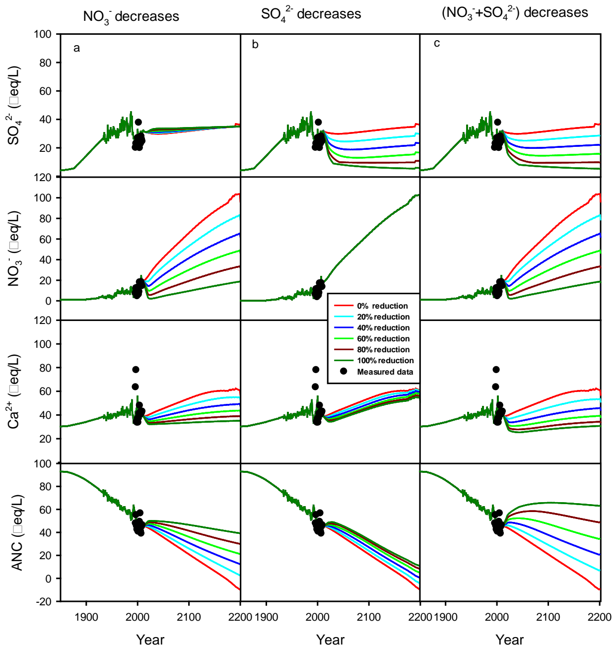
Time series of \text{SO}_4^{2-} , \text{NO}_3^- , \text{Ca}^{2+} and ANC for Mill Creek that include hindcast and future projections to atmospheric deposition decreases in a) \text{NO}_3^- only; b) \text{SO}_4^{2-} only; c) combination of (\text{NO}_3^- + \text{SO}_4^{2-}) . Also shown are measured values.
