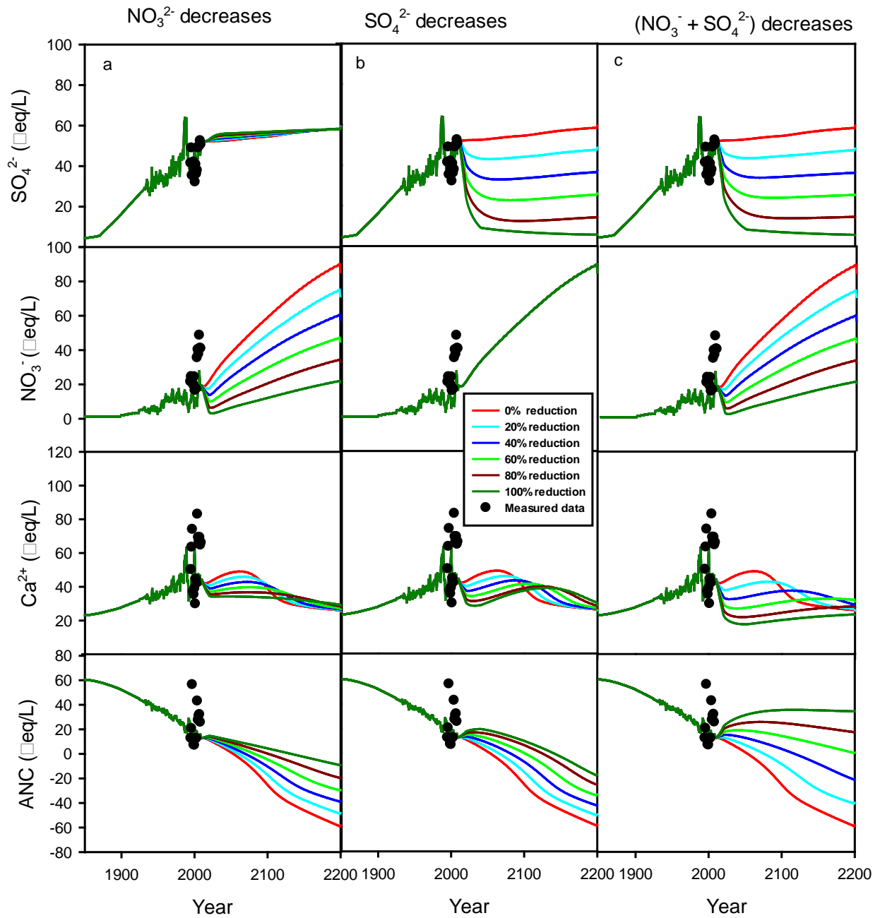
Time series of \text{SO}_4^{2-} , \text{NO}_3^- , \text{Ca}^{2+} and ANC for Cannon Creek that include hindcast and future projections to atmospheric deposition decreases in a) \text{NO}_3^- only; b) \text{SO}_4^{2-} only; c) Combination of (\text{NO}_3^- + \text{SO}_4^{2-}) . Also shown are measured values.
