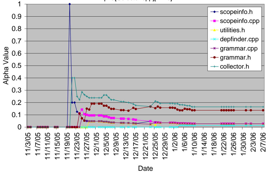
Alpha[Colector.cpp][A file]
